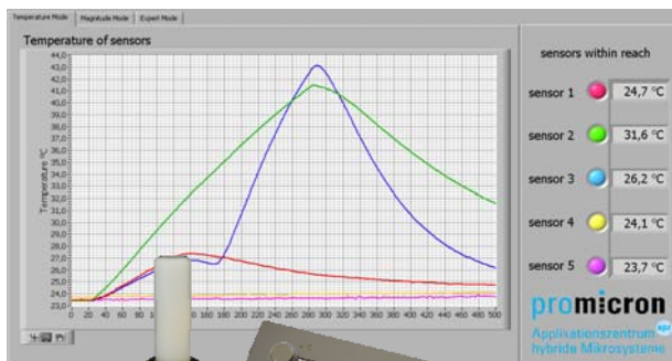
SAW-Sensoren
